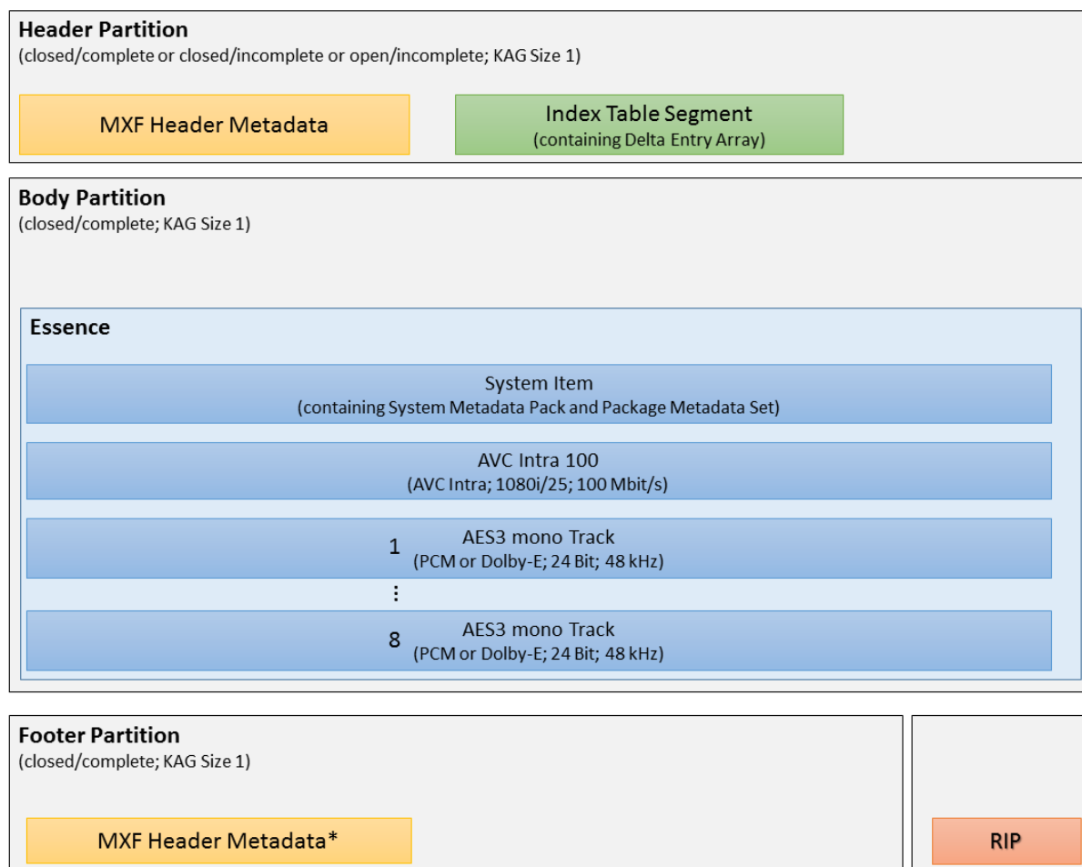
Figure 2 - Structure of the MXF file according to MXF-Profile ARD_ZDF_HDF02a
